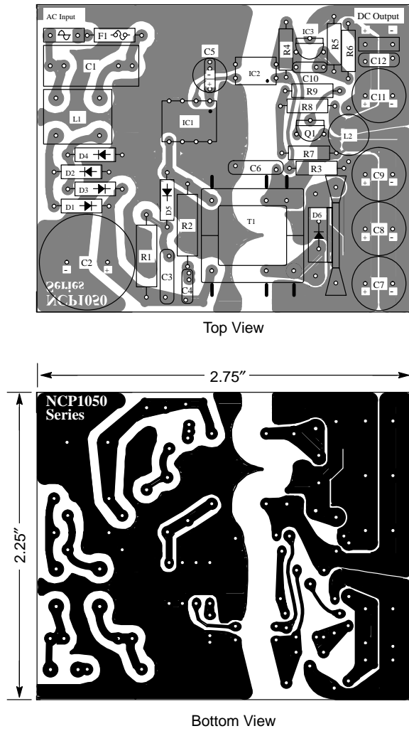
Figure 40. Printed Circuit Board and Component Layout
