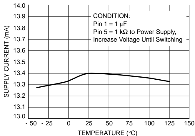
Figure 27. Minimum Startup Drain Voltage versus Temperature
