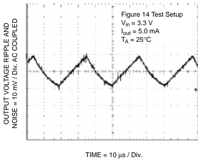
Figure 10. Output Voltage Ripple and Noise
