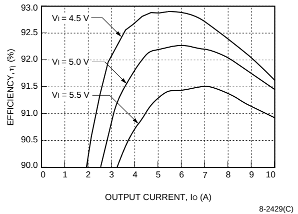
Figure 23. NH033F-L Efficiency, T_A = 25^\circ\text{C}
