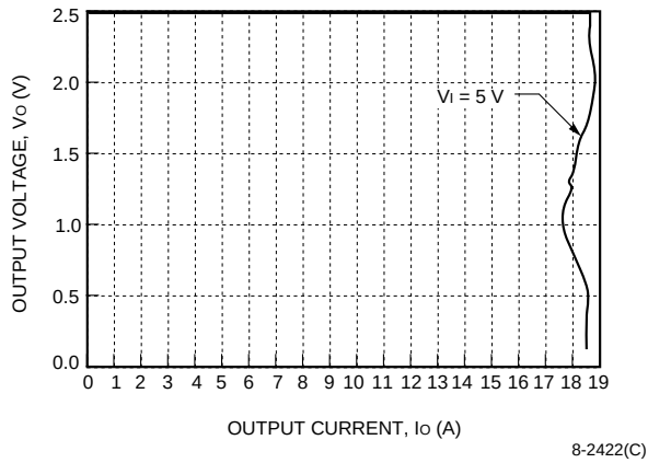
Figure 13. NH033G-L Current Limit, T_A = 25^\circ\text{C}
