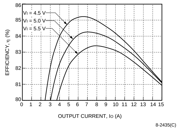
Figure 18. NH050M-L Efficiency, T_A = 25^\circ\text{C}
