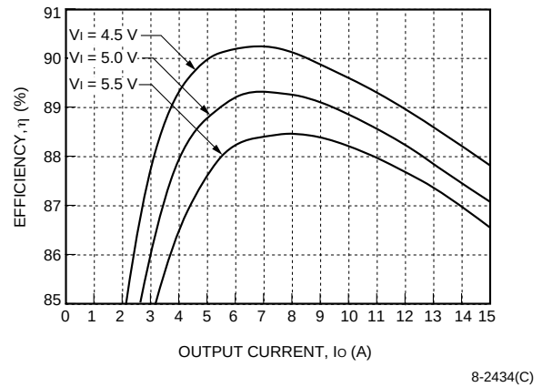
Figure 22. NH050G-L Efficiency, T_A = 25^\circ\text{C}
