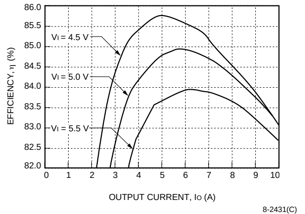
Figure 17. NH033M-L Efficiency, T_A = 25^\circ\text{C}
