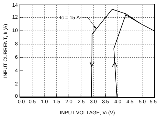
Figure 8. NH050F-L Input Characteristics, T_A = 25^\circ\text{C}
