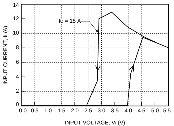
Figure 6. NH050G-L Input Characteristics, T_A = 25\text{ }^{\circ}\text{C}
