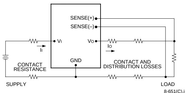
Figure 39. Effective Circuit Configuration for Single-Module Remote-Sense Operation
