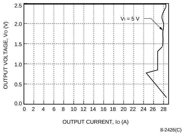
Figure 14. NH050G-L Current Limit, T_A = 25^\circ\text{C}
