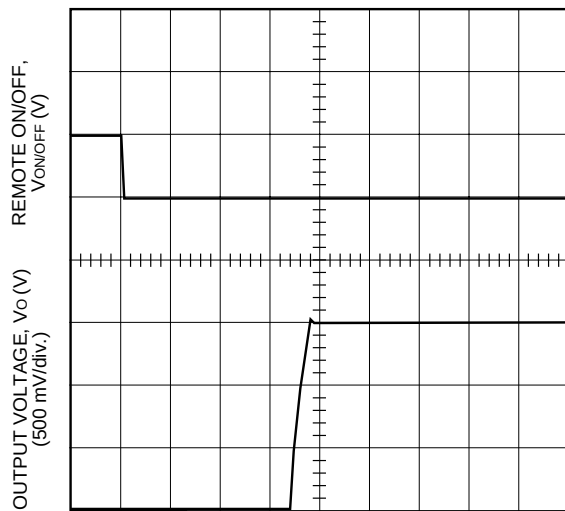
Figure 25. NH033M-L Typical Start-Up from Remote On/Off, V_i = 5 V, I_o = 10 A
