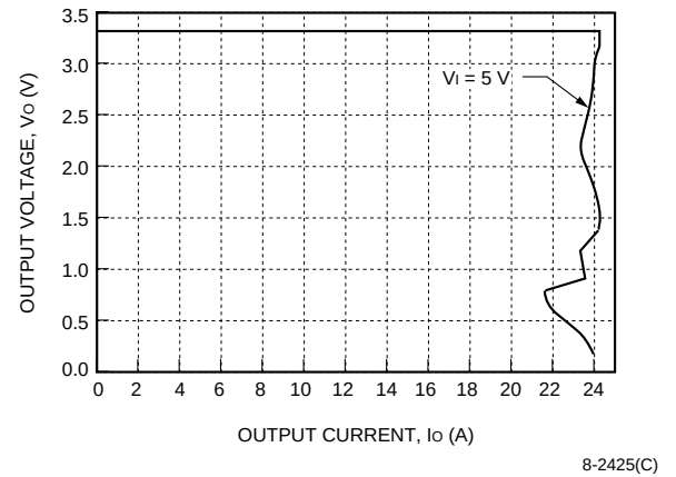
Figure 16. NH050F-L Current Limit, T_A = 25^\circ\text{C}
