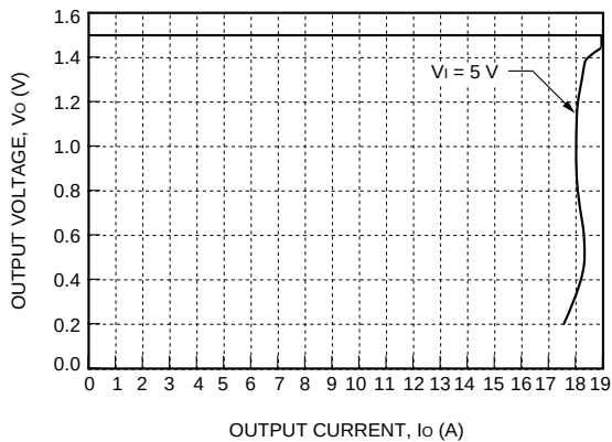
Figure 9. NH033M-L Current Limit, T_A = 25^\circ\text{C}
