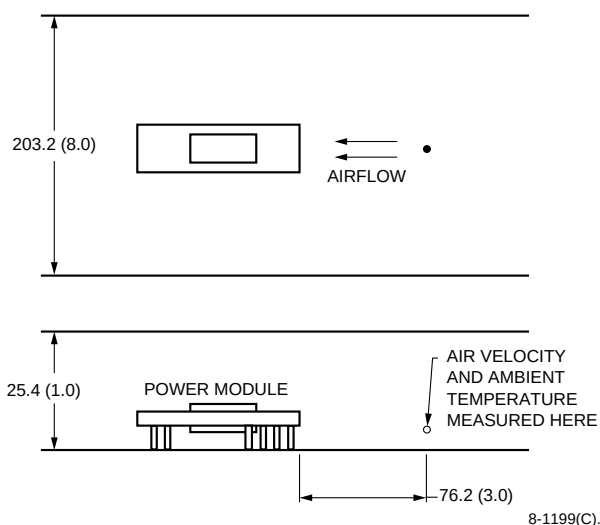
Figure 40. Thermal Test Setup
