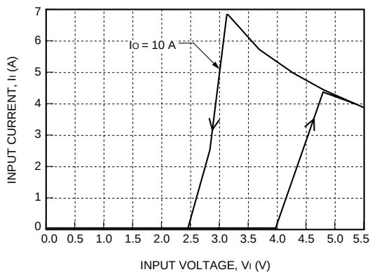
Figure 3. NH033S1R8-L Input Characteristics, T_A = 25\text{ }^{\circ}\text{C}
