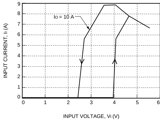
Figure 7. NH033F-L Input Characteristics, T_A = 25^\circ\text{C}
