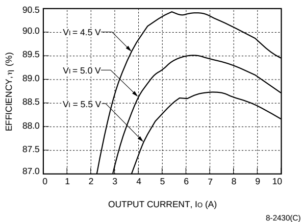
Figure 21. NH033G-L Efficiency, T_A = 25^\circ\text{C}
