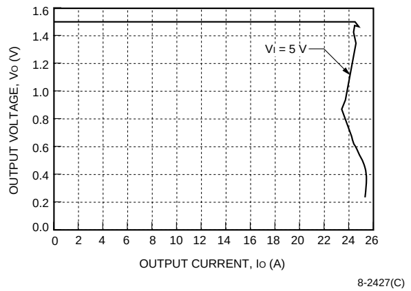
Figure 10. NH050M-L Current Limit, T_A = 25^\circ\text{C}
