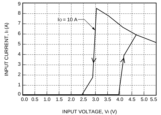
Figure 5. NH033G-L Input Characteristics, T_A = 25\text{ }^{\circ}\text{C}
