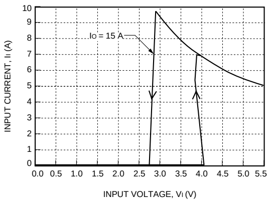
Figure 2. NH050M-L Input Characteristics, T_A = 25\text{ }^{\circ}\text{C}
