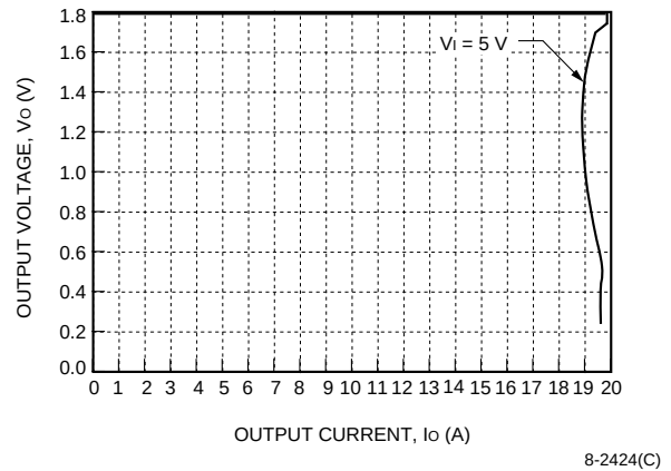
Figure 11. NH033S1R8-L Current Limit, T_A = 25^\circ\text{C}
