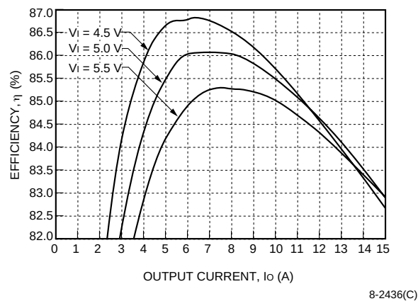
Figure 20. NH050S1R8-L Efficiency, T_A = 25^\circ\text{C}
