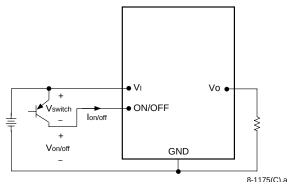
Figure 38. Remote On/Off Implementation
