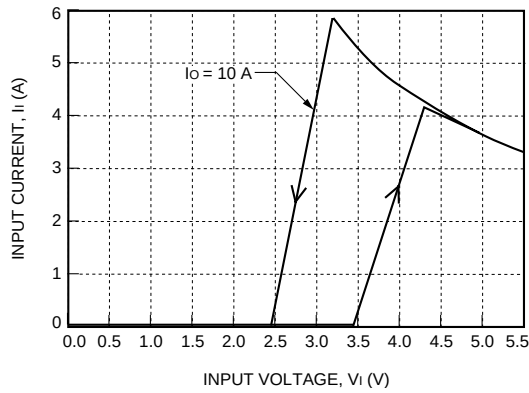
Figure 1. NH033M-L Input Characteristics, T_A = 25\text{ }^{\circ}\text{C}
