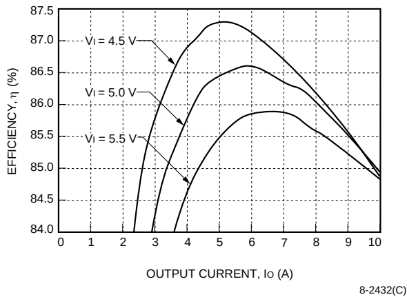
Figure 19. NH033S1R8-L Efficiency, T_A = 25^\circ\text{C}
