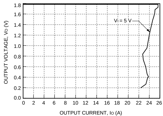
Figure 12. NH050S1R8-L Current Limit, T_A = 25^\circ\text{C}
