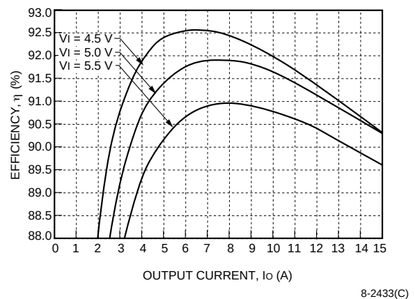
Figure 24. NH050F-L Efficiency, T_A = 25^\circ\text{C}
