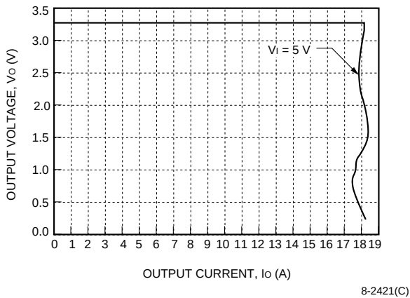
Figure 15. NH033F-L Current Limit, T_A = 25^\circ\text{C}
