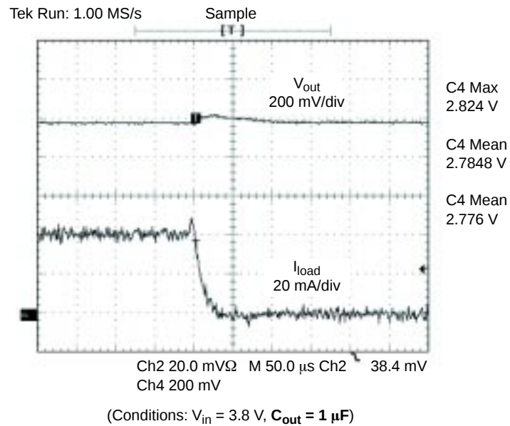
Figure 15. Load Current is Switched from 40 to 0 mA
