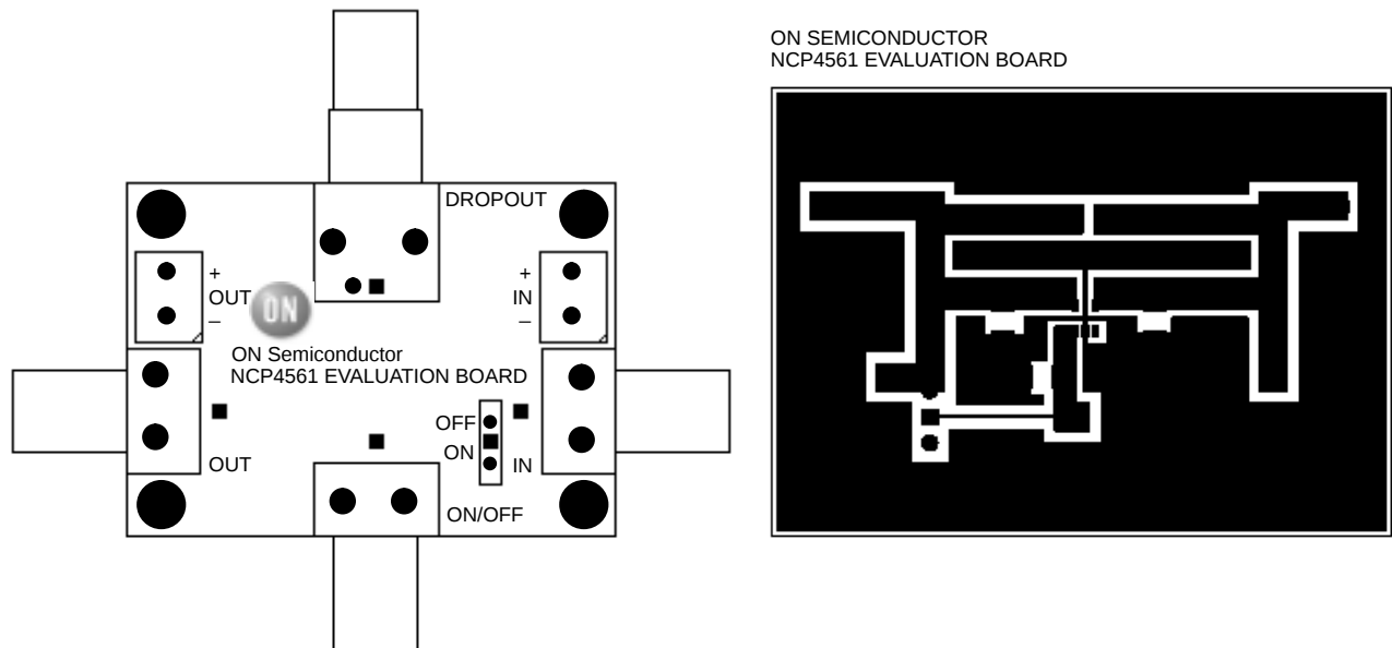
Figure 11. PCB Layout
