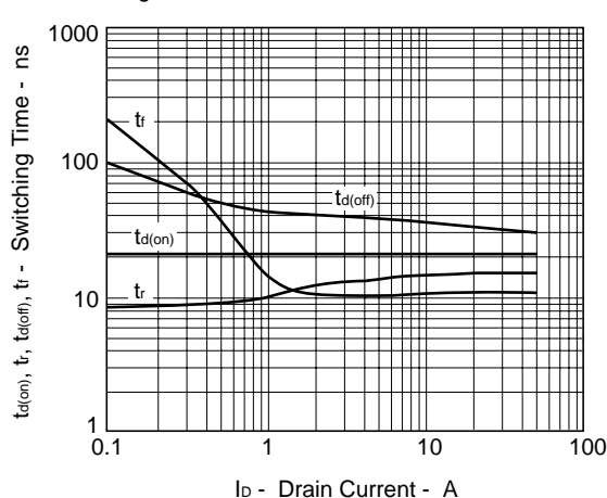
Figure15. SWITCHING CHARACTERISTICS
