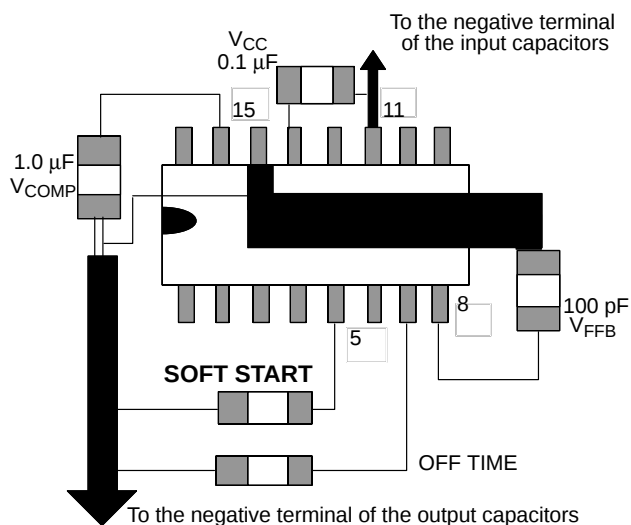
Figure 22. Layout Guidelines
