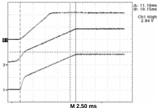
Figure 4. NCP5162 Startup in Response to Increasing 12 V and 5.0 V Input Voltages. Extended Off Time is Followed by Normal Off Time Operation when Output Voltage Achieves Regulation to the Error Amplifier Output
