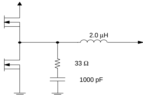
Figure 20. Filter Components
