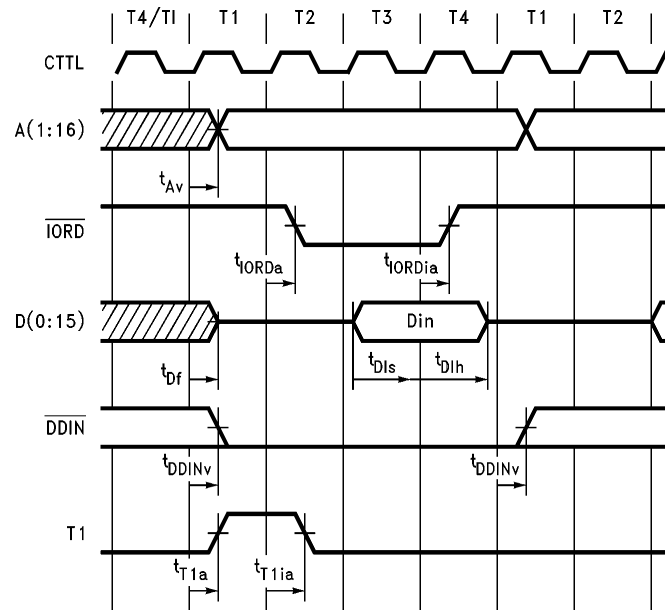
FIGURE 4-11b. I/O Read Cycle
