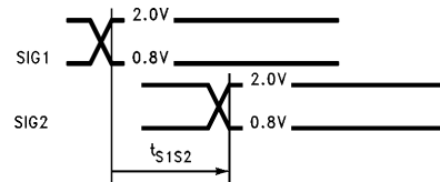
FIGURE 4-4. Asynchronous Signals Specification
