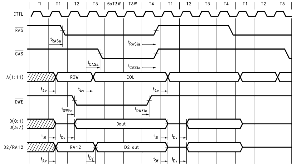
FIGURE 4-5c. DRAM Write Cycle Timing (Internal ROM Mode Only)
