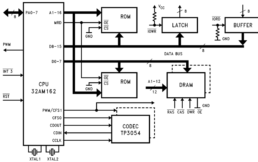
FIGURE 1-2. NS32AM162—External ROM Mode
