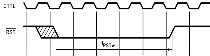
FIGURE 4-16. Non Power On Reset
