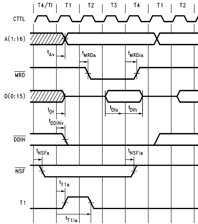
FIGURE 4-11a. External Memory Read Timing
