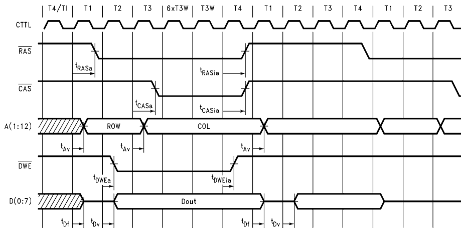
FIGURE 4-5d. DRAM Write Cycle Timing (External ROM or Development Modes)
