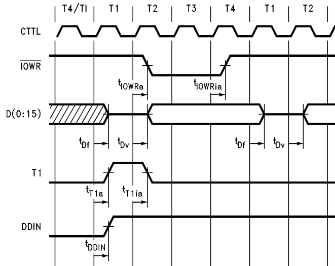
FIGURE 4-12b. I/O Write Cycle Timing
