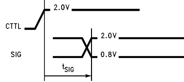
FIGURE 4-2. Synchronous Output Signals Specification
