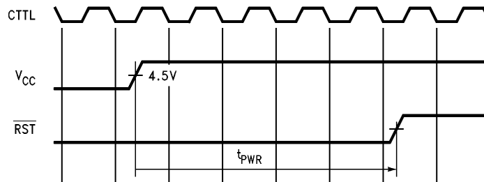
FIGURE 4-17. Power On Reset
