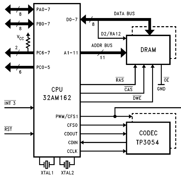
FIGURE 1-1. NS32AM162—Internal ROM Mode
