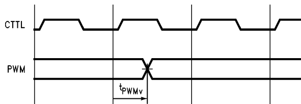
FIGURE 4-13b. PWM Output Timing
