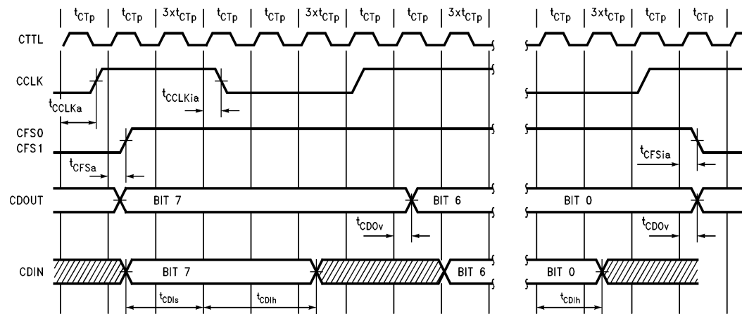
FIGURE 4-8. CODEC Long Frame Timing, 8 KHz Sampling Rate
