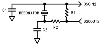
FIGURE 3-10. Low Frequency Resonator Connections
