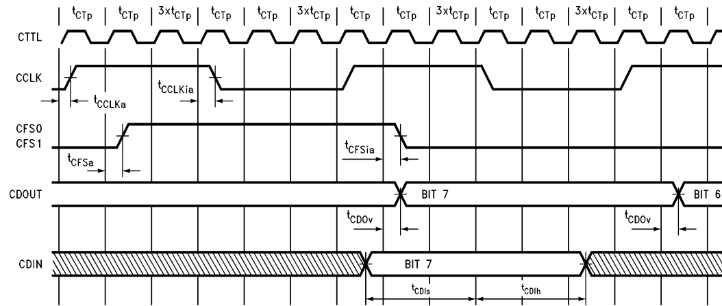
FIGURE 4-9. CODEC Short Frame Timing, 8 KHz Sampling Rate
