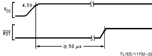
FIGURE 3-12. Power-On Reset Requirements
