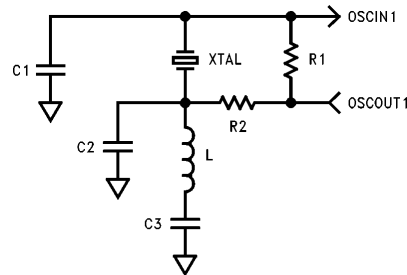
FIGURE 3-9. High Frequency Crystal Connections
