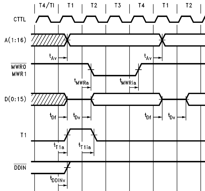
FIGURE 4-12a. External Memory Write—Cycle Timing
