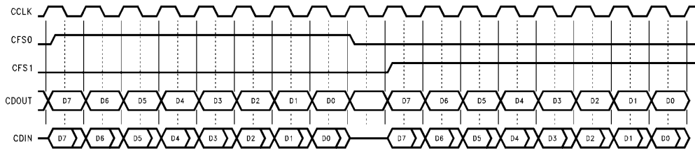
FIGURE 3-7. CODEC Protocol—Long Frame
