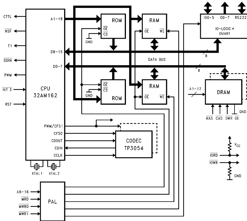
FIGURE 1-3. NS32AM162—Development Mode
