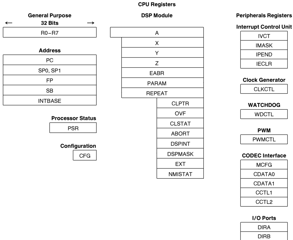
FIGURE 2-1. NS32AM162 Internal Registers
