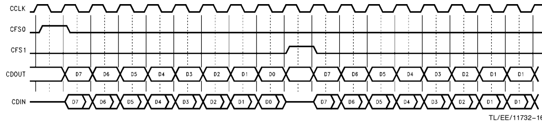
FIGURE 3-6. CODEC Protocol—Short Frame
