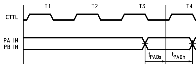
FIGURE 4-14. Port A and Port B Input Timing
