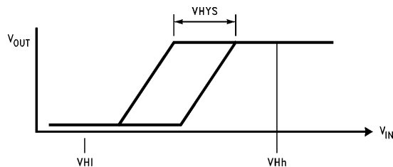
FIGURE 4-4b. Hysteresis Inputs Definition
