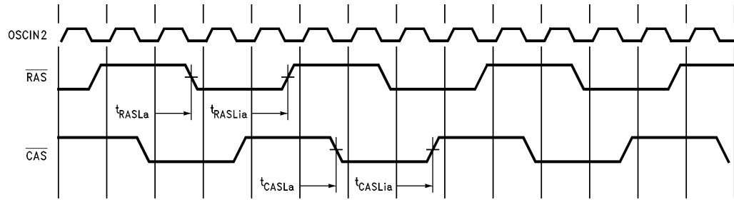
FIGURE 4-7. DRAM Power Down Refresh
