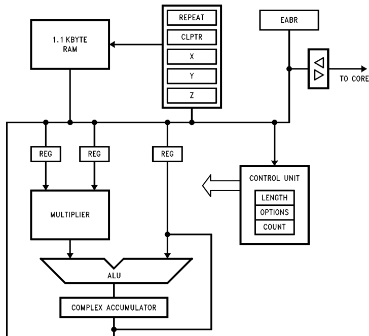
FIGURE 3-8. DSP Module Block Diagram
