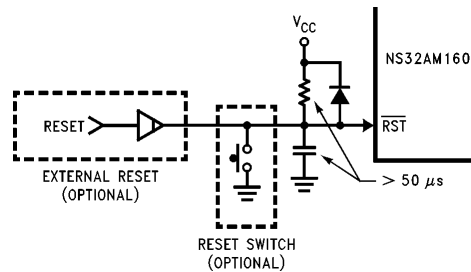
FIGURE 3-11. Recommended Reset Connections
