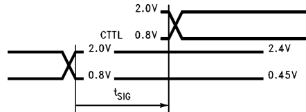
FIGURE 4-3. Synchronous Input Signals Specification
