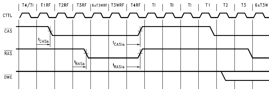
FIGURE 4-6. DRAM Refresh Cycle Timing (In Normal Operation Mode)
