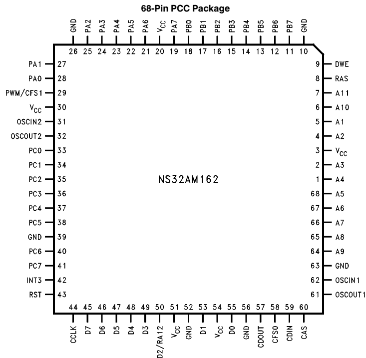
FIGURE 4-1. Connection Diagram
