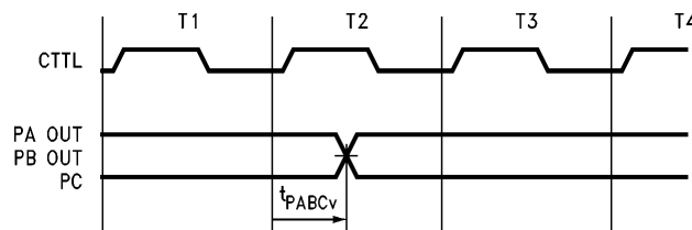
FIGURE 4-13a. Port A, Port B and Port C Timing
