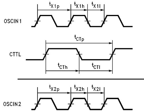
FIGURE 4-15. CTTL, OSCIN1 and OSCIN2 Timing
