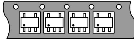
Figure 8. SOT-353/SC70-5/SC-88A Reel Configuration/Orientation
