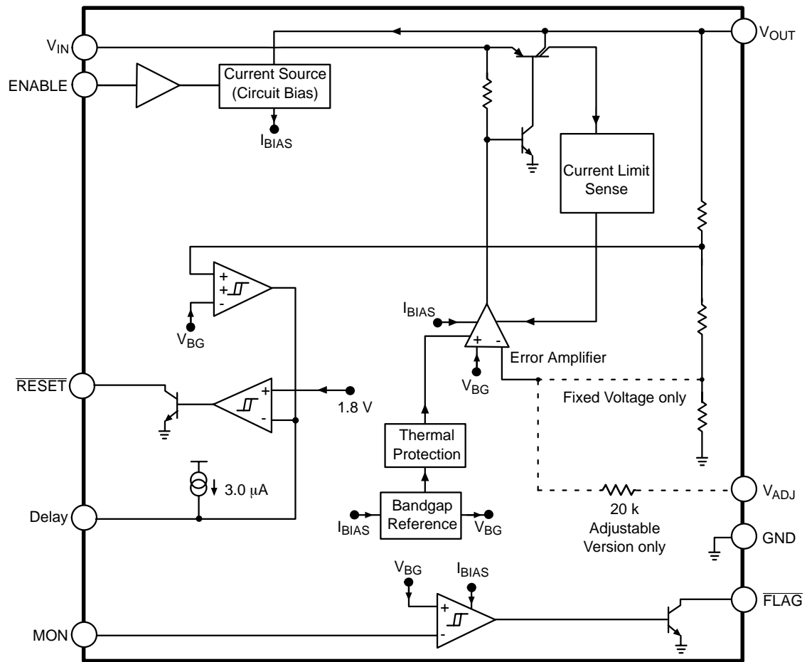
Figure 11. Block Diagram
