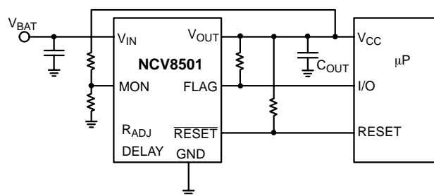
Figure 14. Flag/Monitor Function
