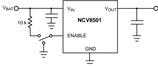
Figure 13. ENABLE Function
