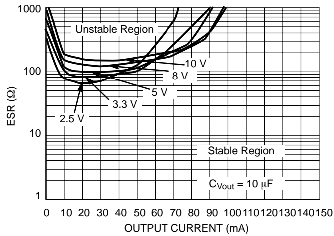
Figure 10. Output Capacitor ESR
