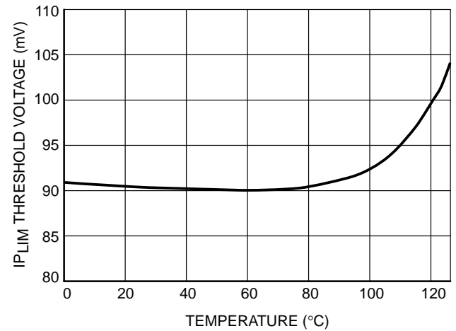
Figure 14. I_{PLIM} Threshold versus Temperature
