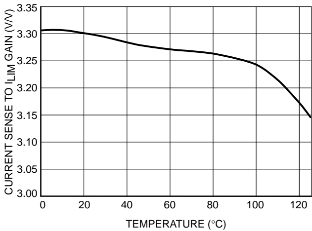
Figure 13. CS Amp to I_{LIM} Gain versus Temperature
