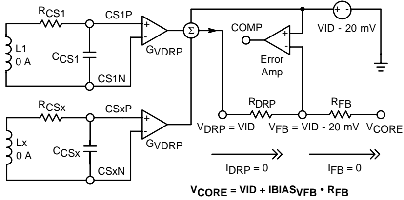
Figure 27. AVP Circuitry at No-Load
