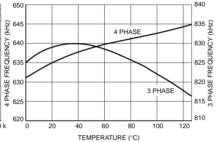
Figure 8. Switching Frequency versus Temperature (ROSC = 32.4 kΩ)
