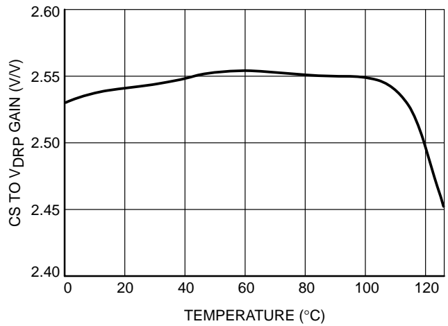
Figure 10. Current Sense to V_{DRP} Gain versus Temperature
