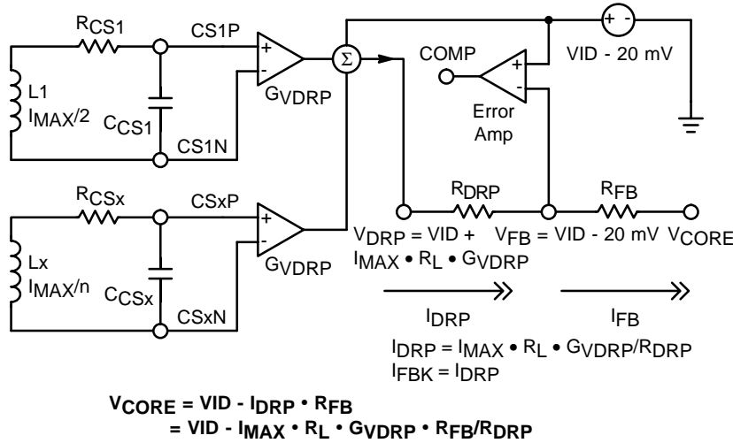
Figure 28. AVP Circuitry at Full-Load
