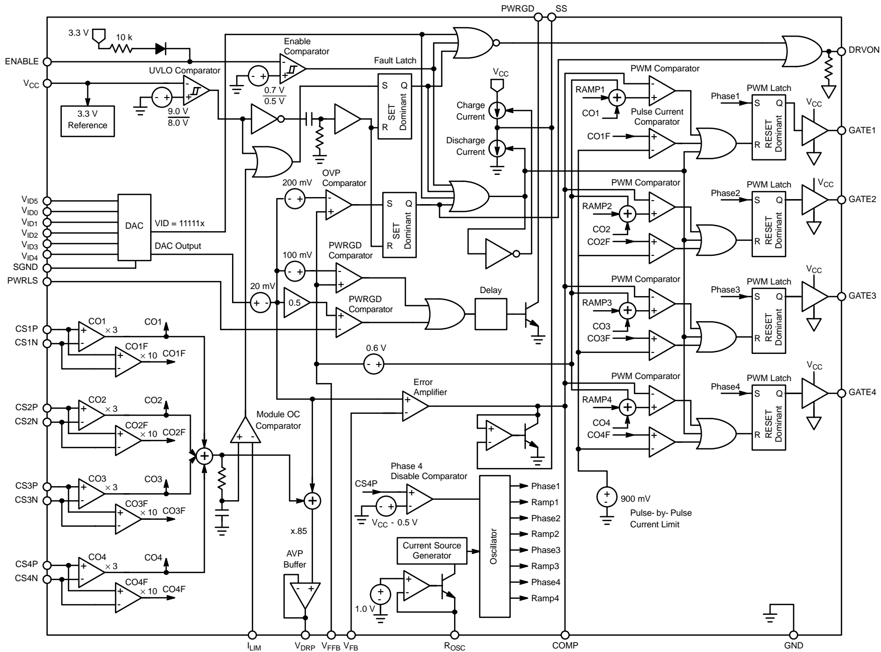
Figure 2. Block Diagram
