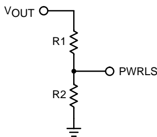
Figure 23. Adjusting the PWRGD Threshold
