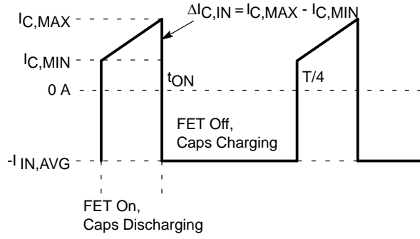
Figure 24. Input Capacitor Current for a Four-Phase Converter
