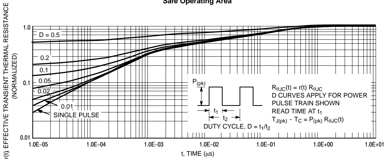
Figure 12. Thermal Response
