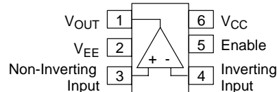
Style 2 Pinout (SN2T1)
