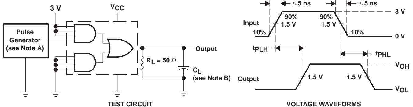
Figure 1. Test Circuit and Voltage Waveforms
