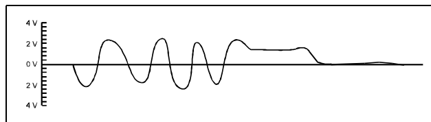
Figure 3. TPO Output Waveform
