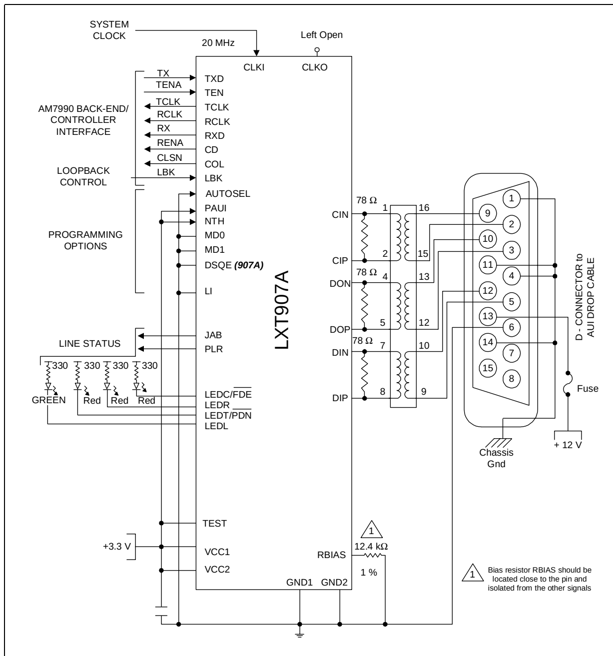
Figure 15. AUl Encoder/Decoder Only Application
