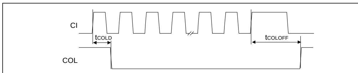
Figure 27. Mode 2 COL/CI Output Timing
