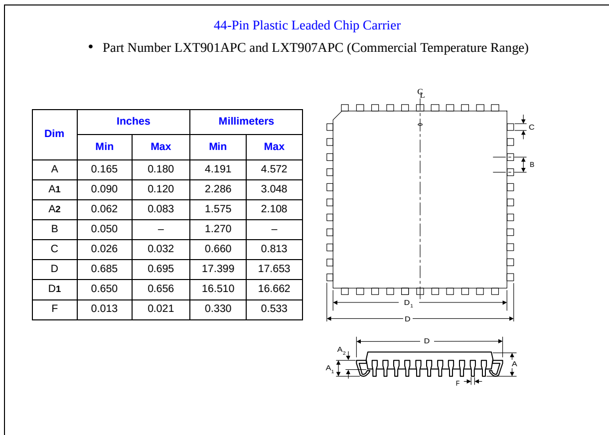
Figure 43. 44-Pin PLCC
