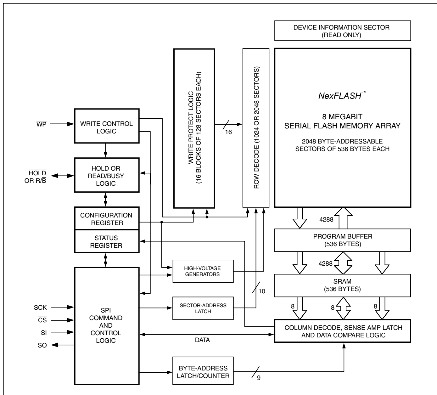
Figure 2. NX25F080A Architectural Block Diagram
