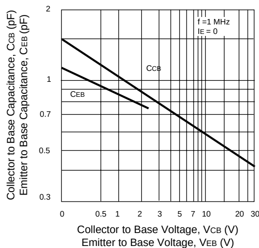
DEVICE CAPACITANCE
