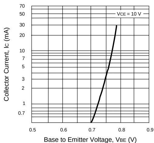
VOLTAGE CURRENT CHARACTERISTICS
