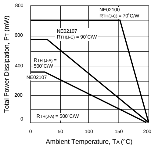
NE02100, NE02107 DC POWER DERATING CURVES
