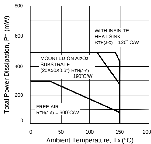
NE02135 DC POWER DERATING CURVES
