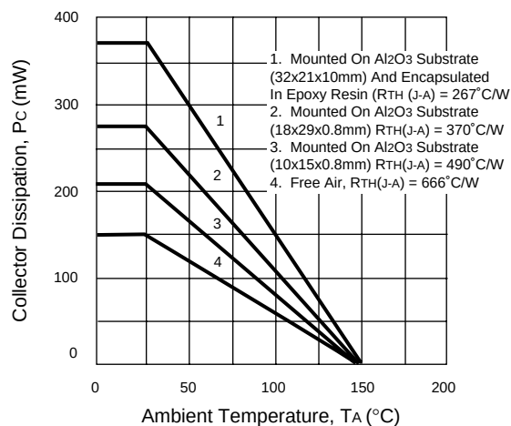
NE02133 DC POWER DERATING CURVES
