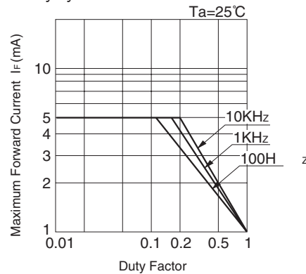
■ Duty Cycle vs. Maximum Forward Current
