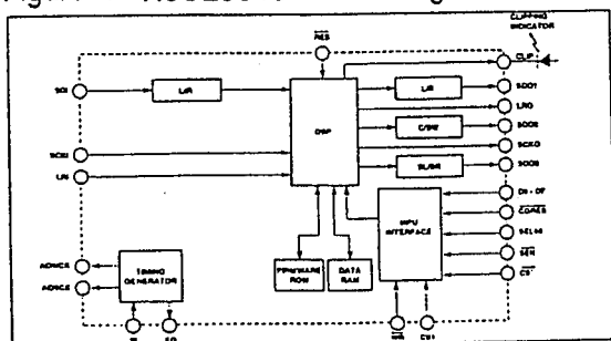
Figure 1 NJU25019 Block Diagram
