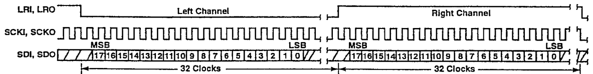
4 Figure 14 I 2 S Data Format, AD\text{SCK} = 64\text{ Fs} , 18-bit Data
