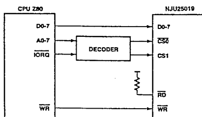
Figure 25 Z80 Interface
