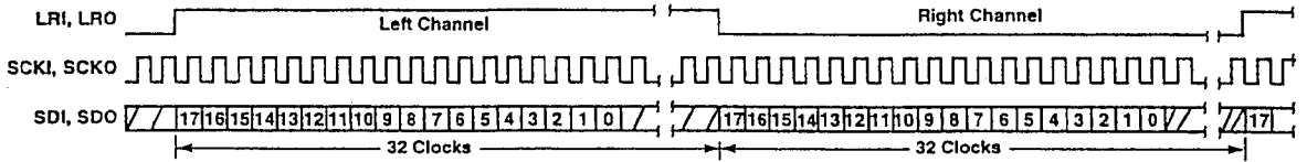
Figure 12 Left-Justified Data Format, AD\text{SCK} = 64\text{ Fs} , 18-bit Data
