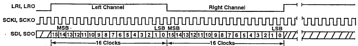
Figure 15 Right- and Left-Justified Data Formats, AD\text{SCK} = 32\text{ Fs} , 16-bit Data
