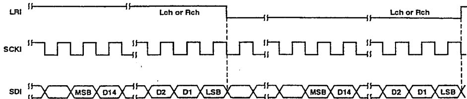
Figure 23 Serial Data Input Format
