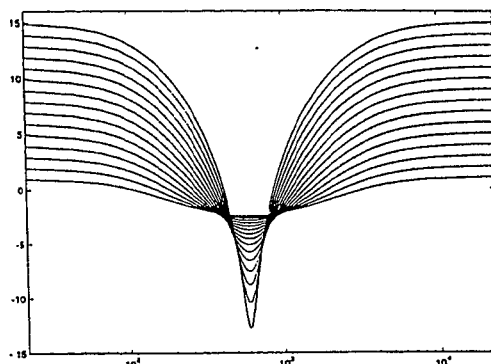
Figure 22 BBE Phase vs. Frequency
