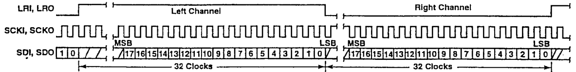
Figure 13 Right-Justified Data Format, AD\text{SCK} = 64\text{ Fs} , 18-bit Data
