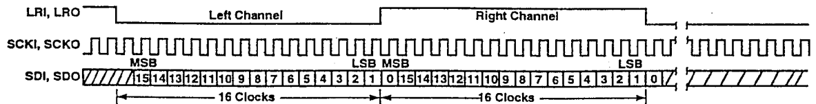
Figure 16 I 2 S Data Formats, AD\text{SCK} = 32\text{ Fs} , 16-bit Data
