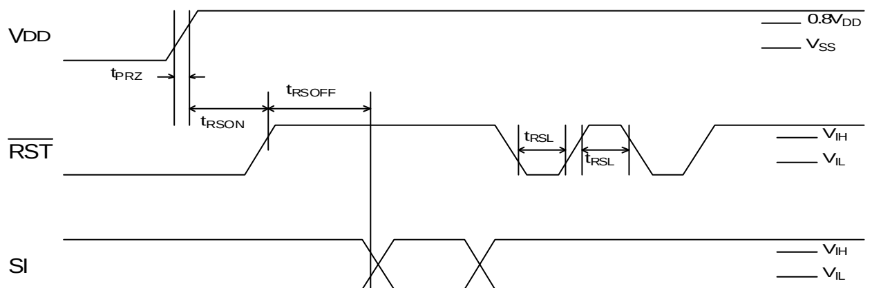
Fig.2 Reset Timing
