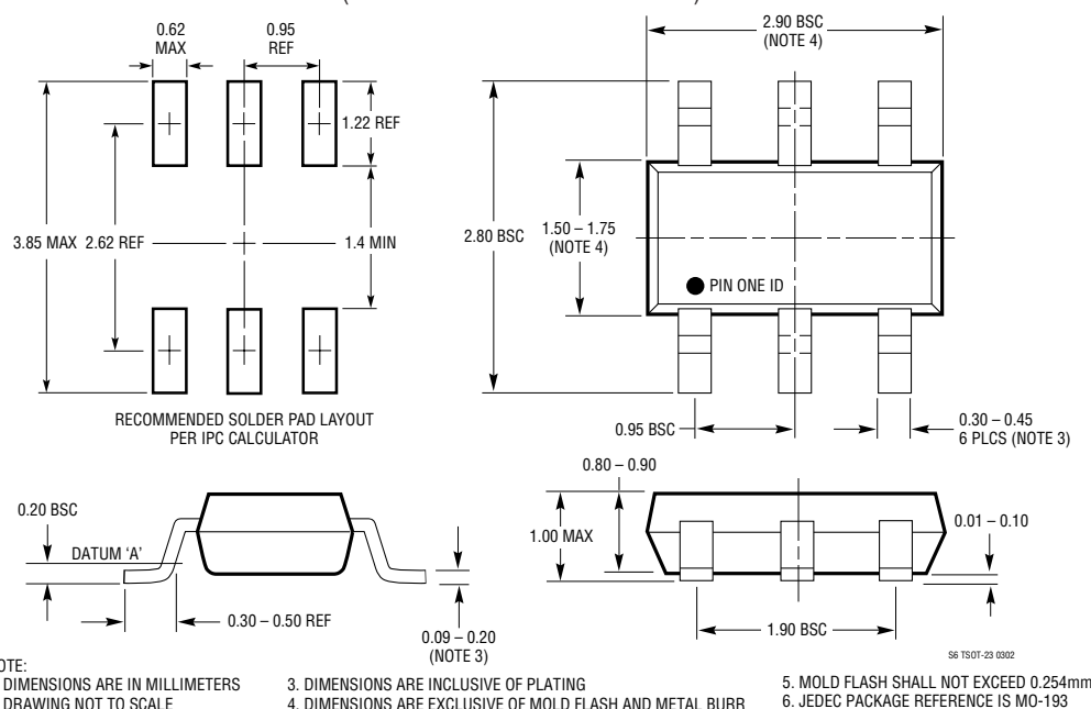
S6 Package 6-Lead Plastic TSOT-23 (Reference LTC DWG # 05-08-1636)
