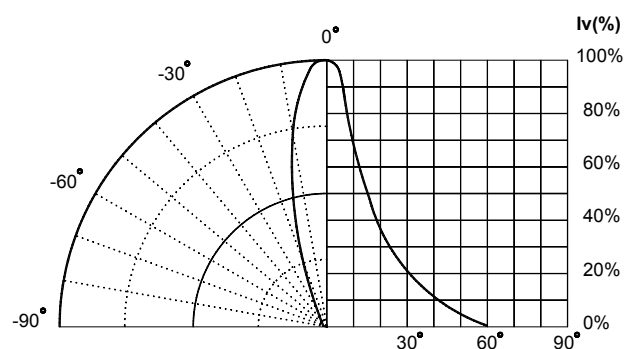
Beam Pattern
