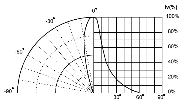
Beam Pattern
