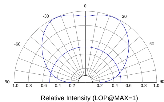
Beam Pattern
