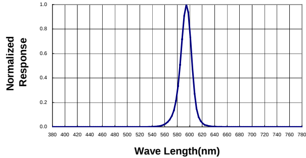
Spectral Radiance ( Peak @ 595nm)
