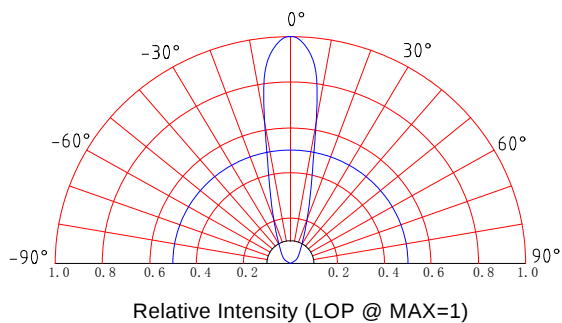
Beam Pattern
