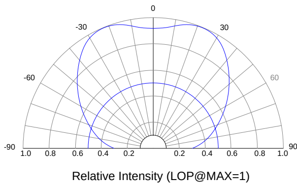
Beam Pattern
