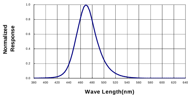
Spectral Radiance (Peak @ 468nm)
