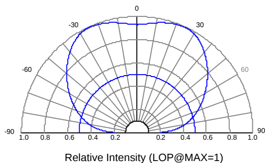
Beam Pattern
