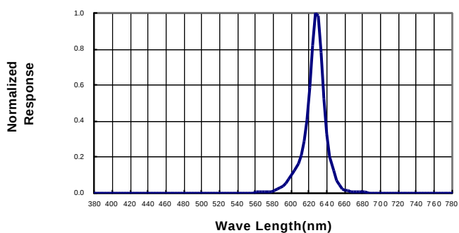
Spectral Radiance (Peak @ 630nm)
