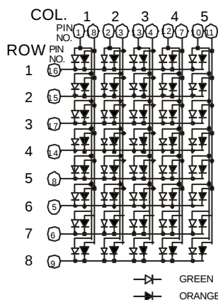
LMD23058C
