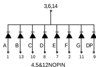
LSD100C
