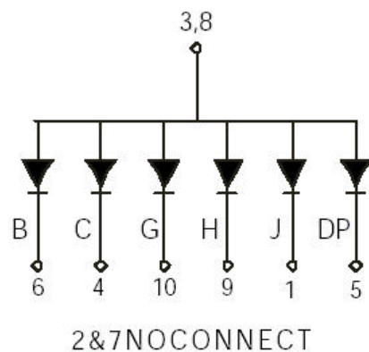
LSD053BG-10
