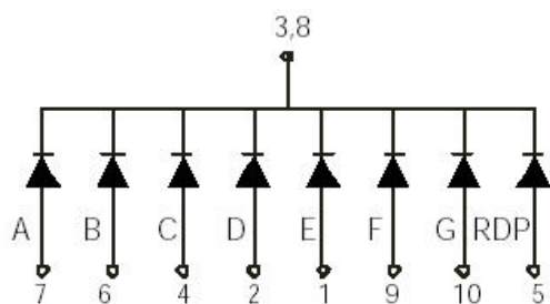
LSD050AG-10
