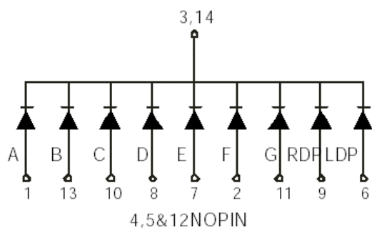
LSD043AG-10
