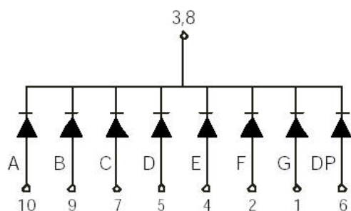
LSD039AG-10
