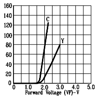
Fig5. FORWARD CURRENT VS. FORWARD VOLTAGE
