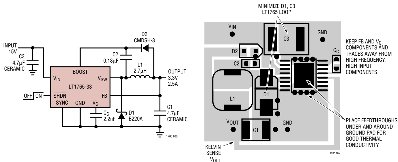
Figure 6. Typical Application and Layout (Topside Only Shown)
