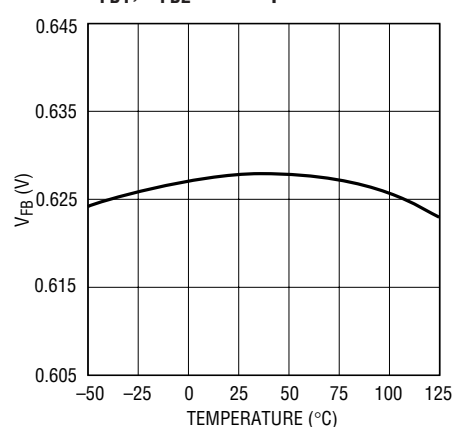
V_{FB1} , V_{FB2} vs Temperature
