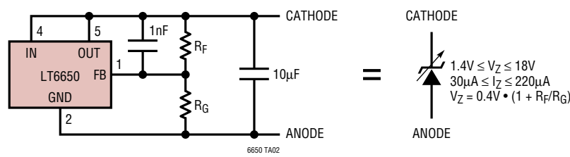
Adjustable Micropower “Zener” 2-Terminal Reference
