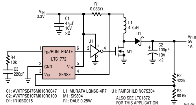
LTC1772 3.3V to 5V/1A Boost Regulator
