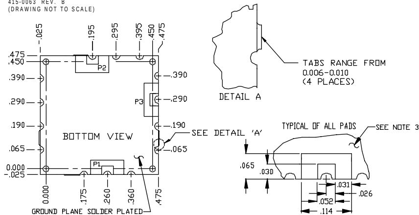
PHYSICAL DIMENSIONS
