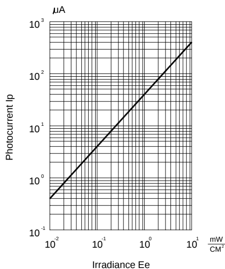
Fig.6 PHOTOCURRENT VS IRRADIANCE \lambda = 940 nm
