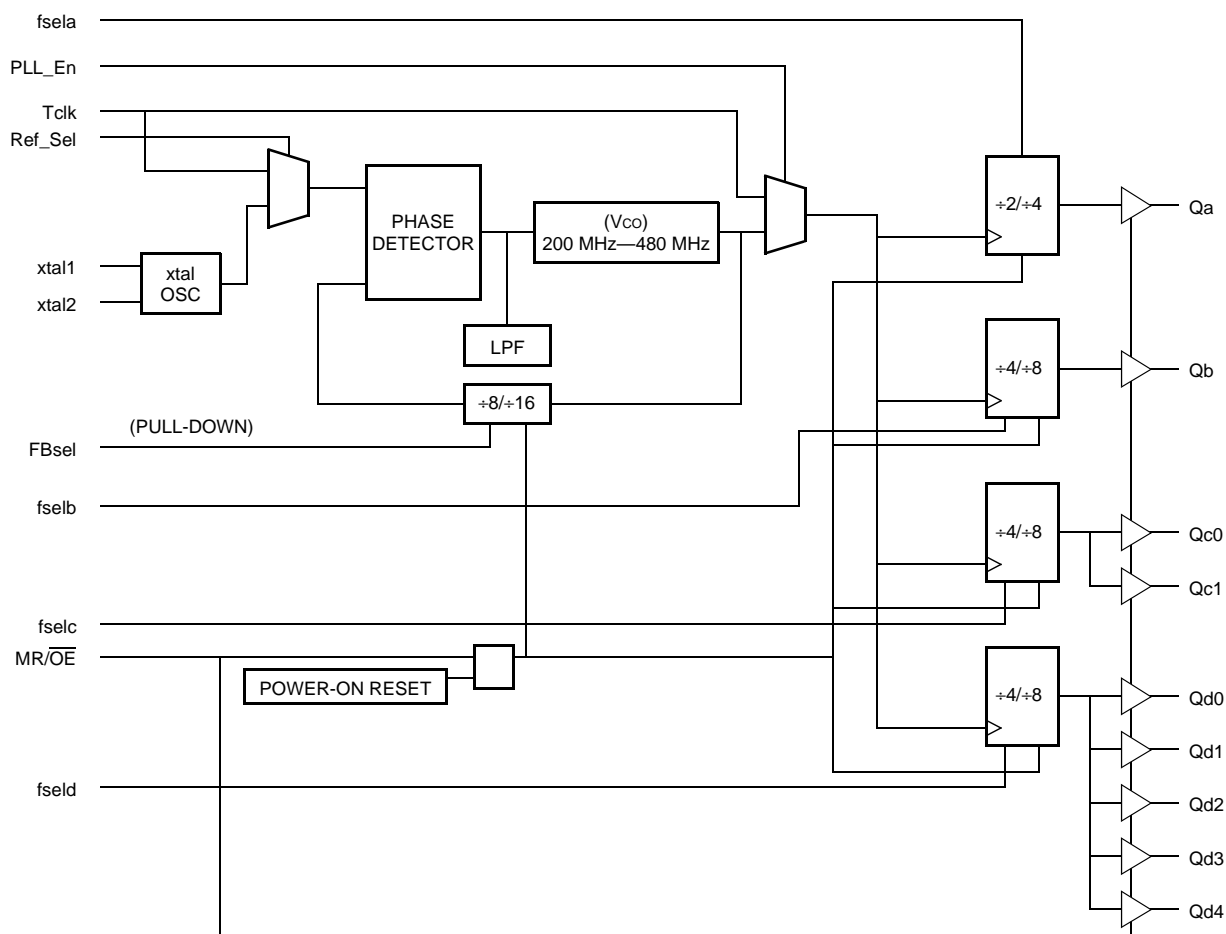
Figure 1. Logic Diagram
