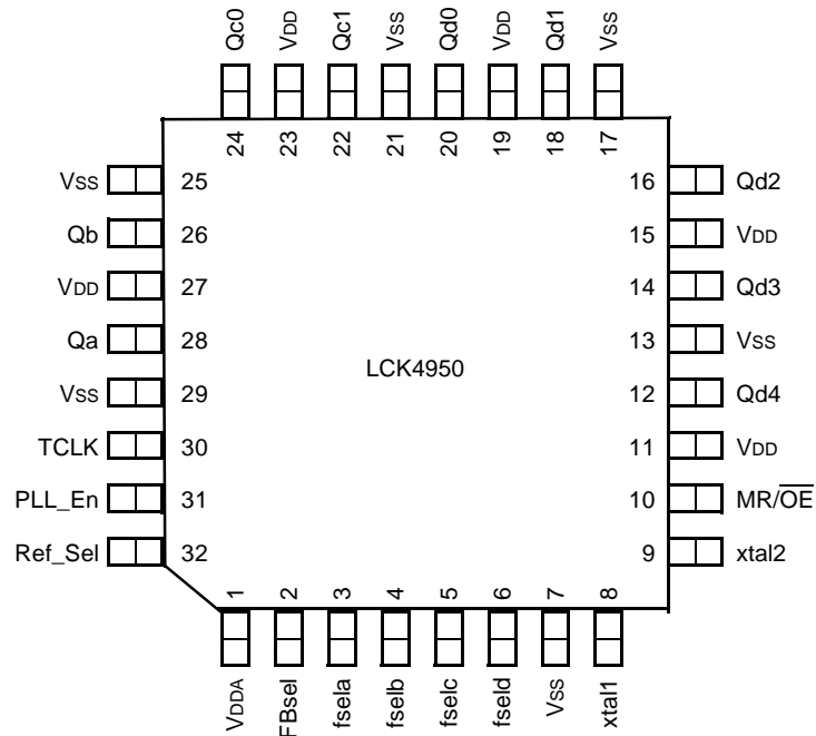
Figure 2. Pin Diagram
