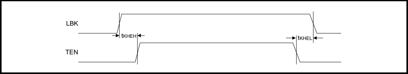
Figure 41: Mode 4 Loopback Timing
