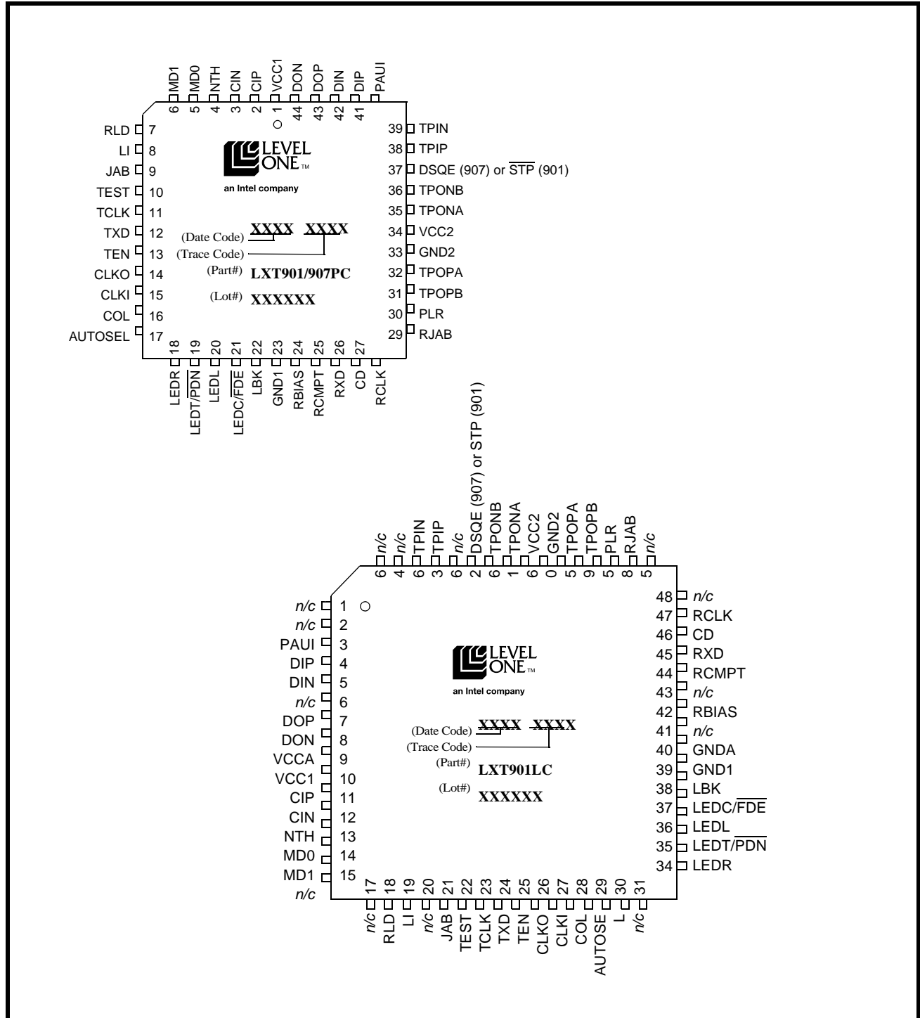
Figure 1: LXT901/907 Pin Assignments
