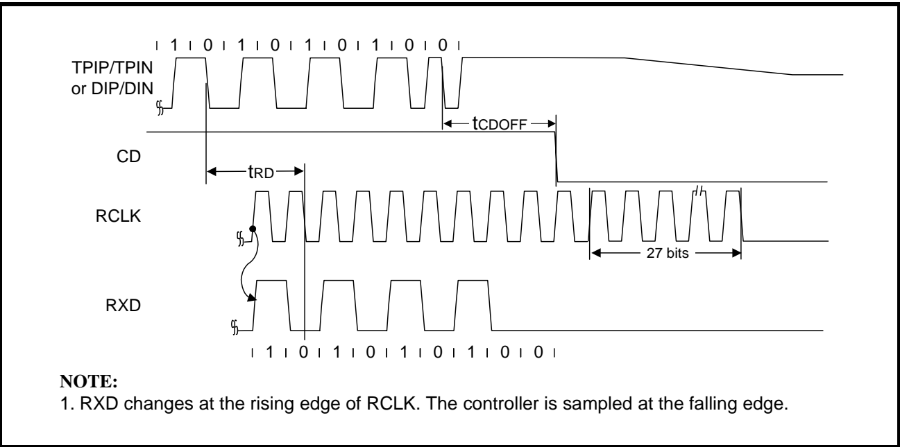
Figure 29: Mode 3 RCLK/End-of-Frame Timing ( LXT901 only )
