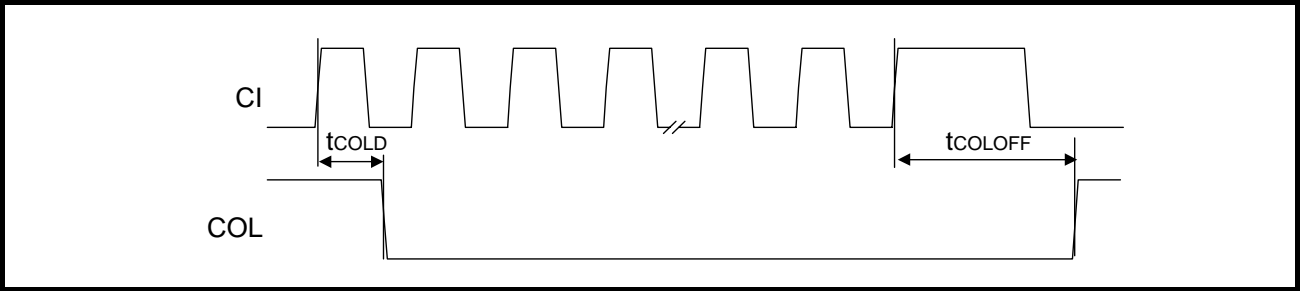
Figure 25: Mode 2 Collision Detect Timing
