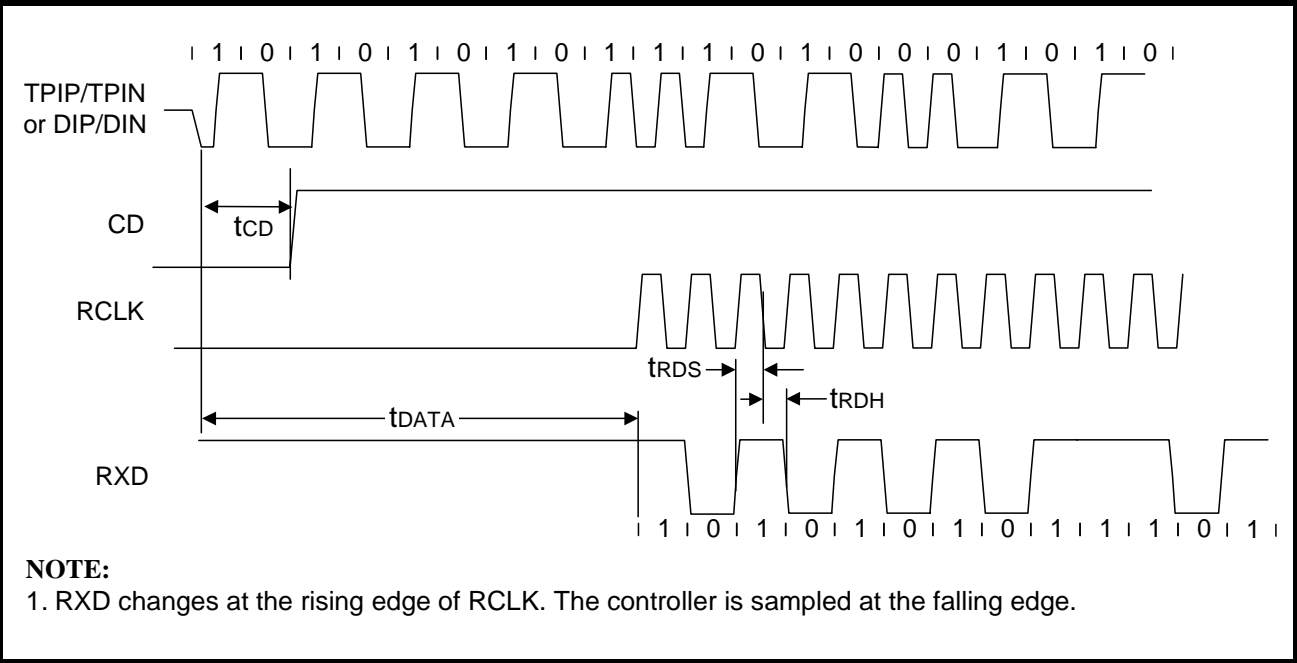
Figure 22: Mode 2 RCLK/Start-of-Frame Timing
