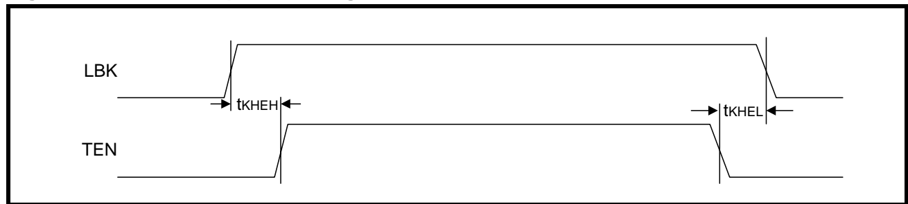
Figure 35: Mode 3 Loopback Timing
