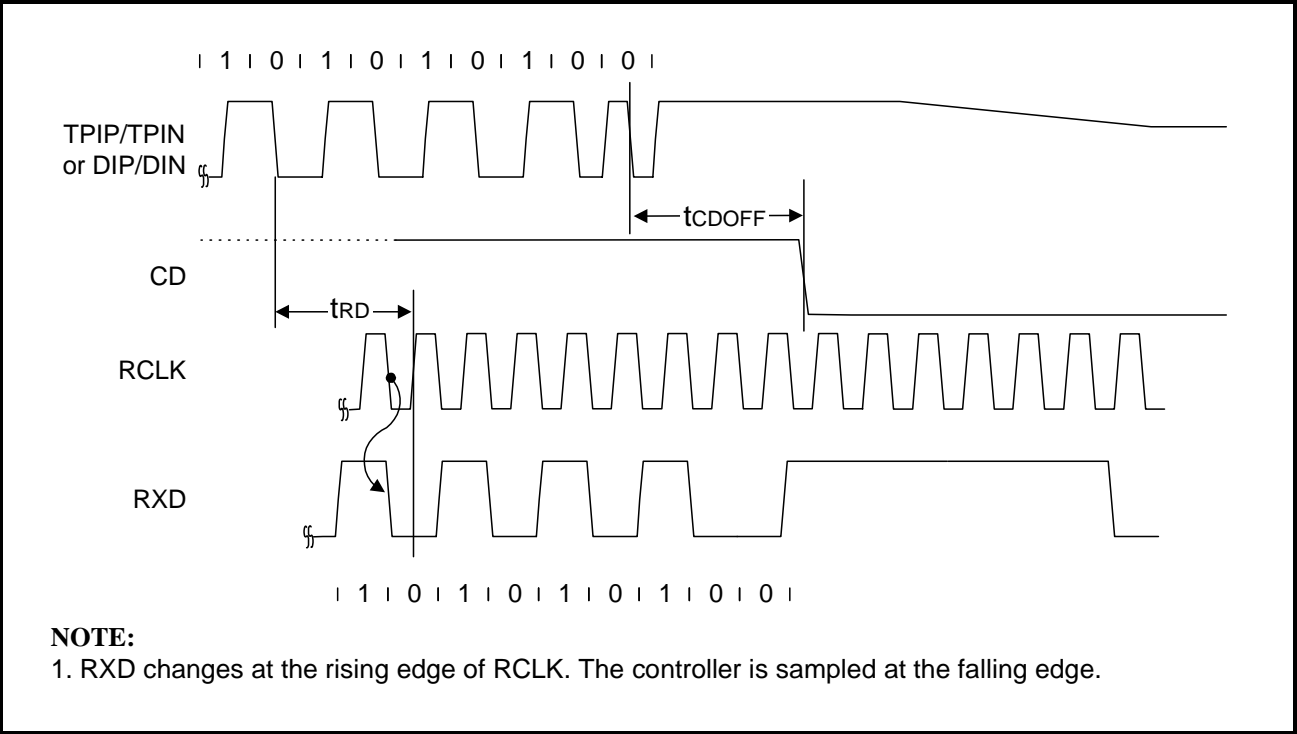
Figure 37: Mode 4 RCLK/End-of-Frame Timing
