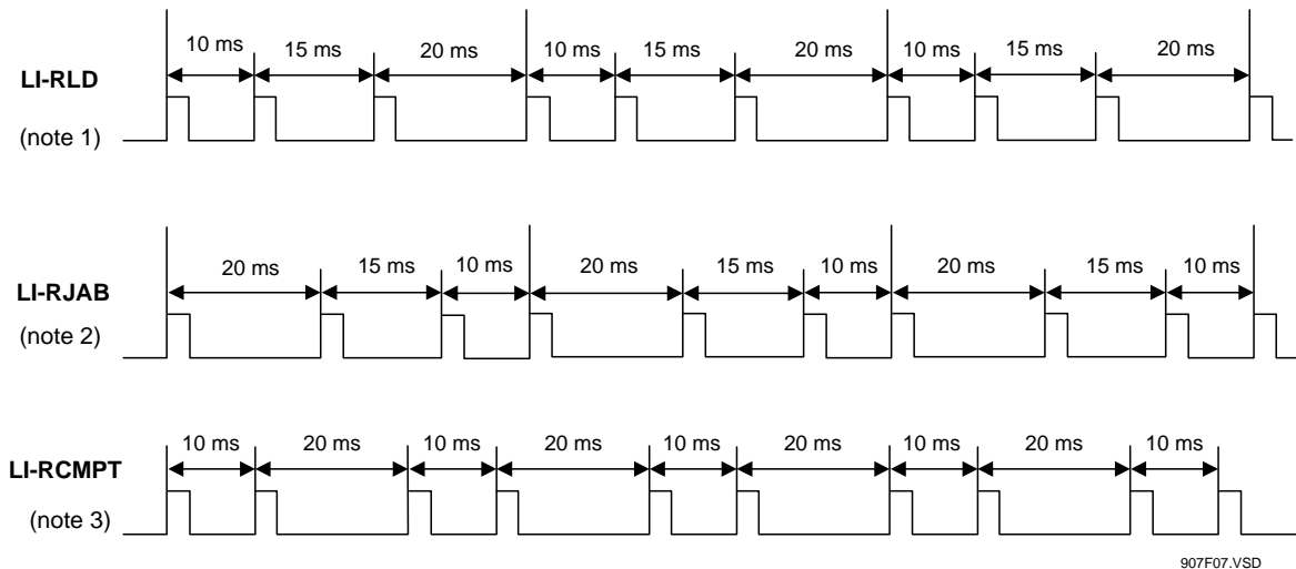
Figure 7: Remote Signaling Link Integrity Pulse Timing
