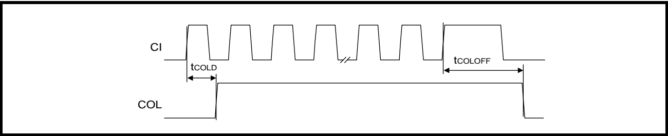
Figure 19: Mode 1 Collision Detect Timing
