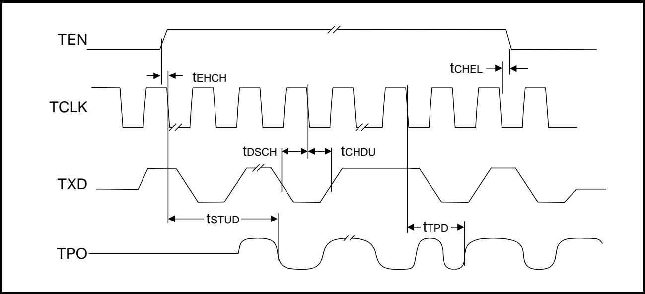
Figure 32: Mode 3 Transmit Timing
