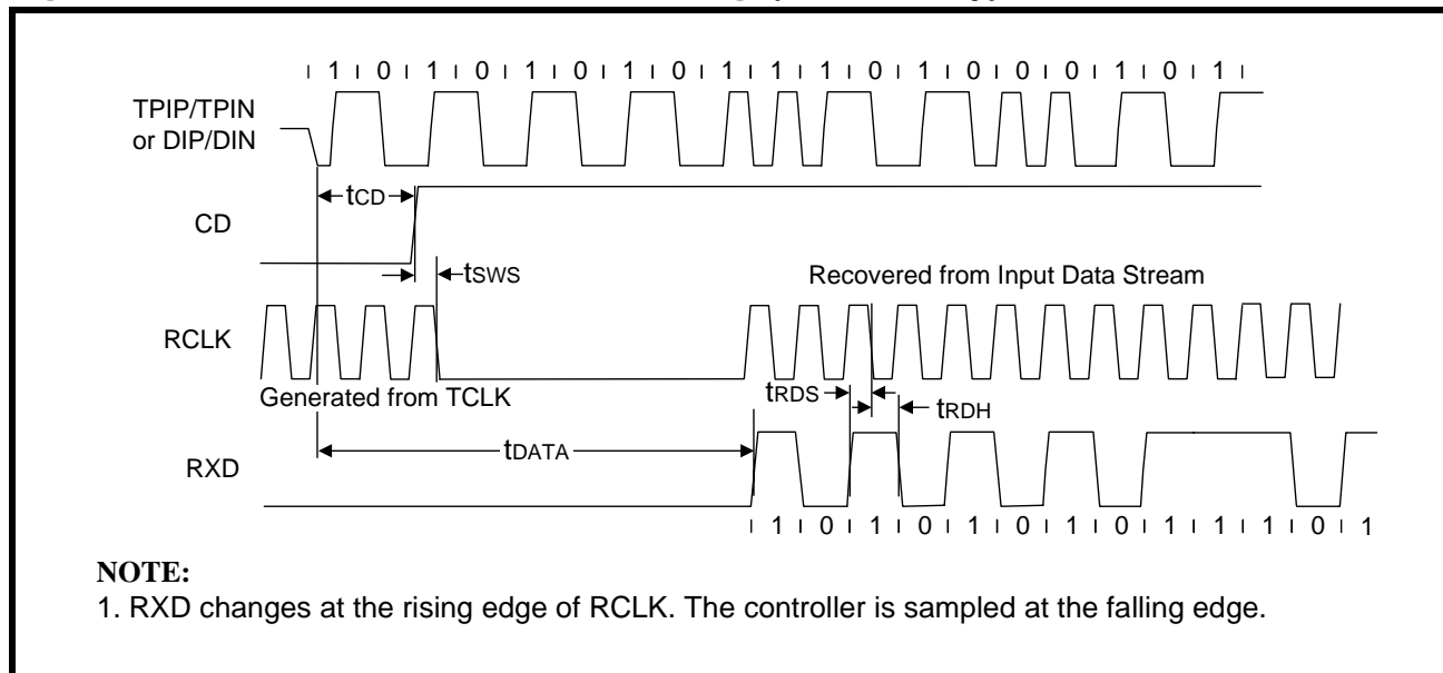
Figure 30: Mode 3 RCLK/Start-of-Frame Timing (LXT907 only)
