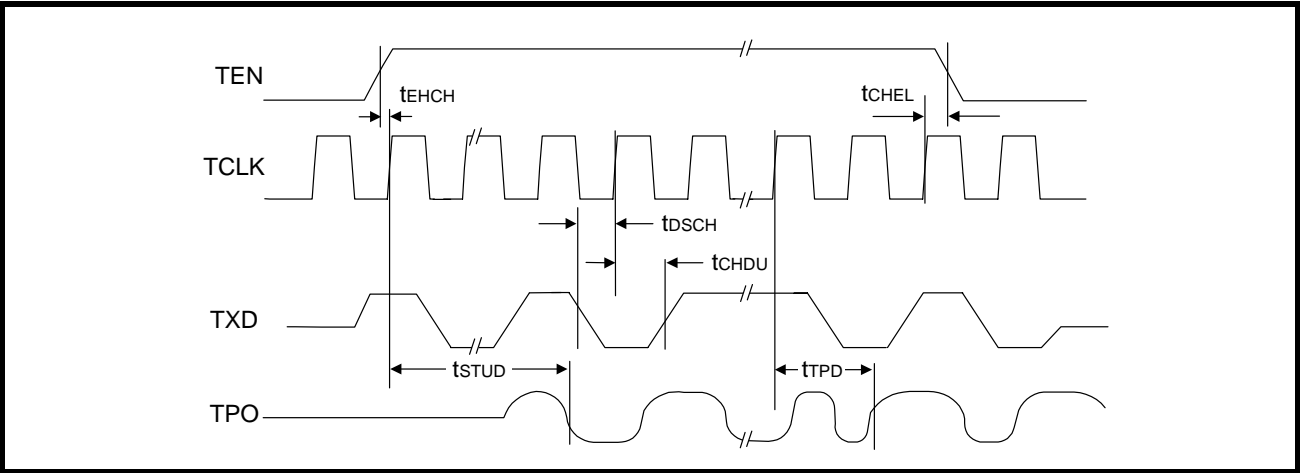
Figure 18: Mode 1 Transmit Timing
