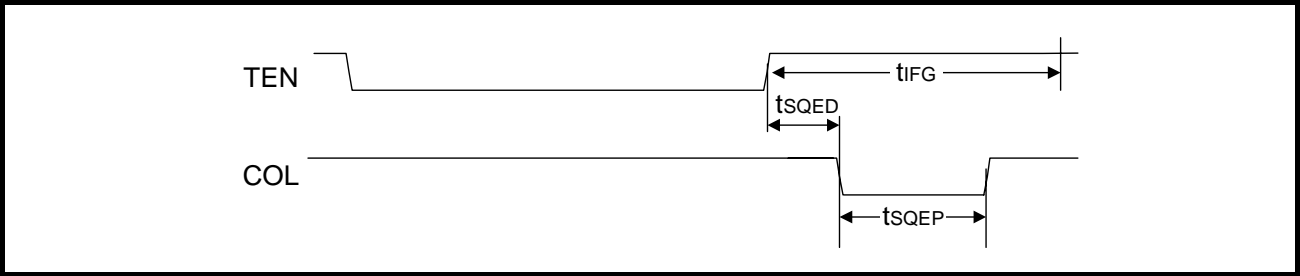
Figure 26: Mode 2 COL/CI Output Timing
