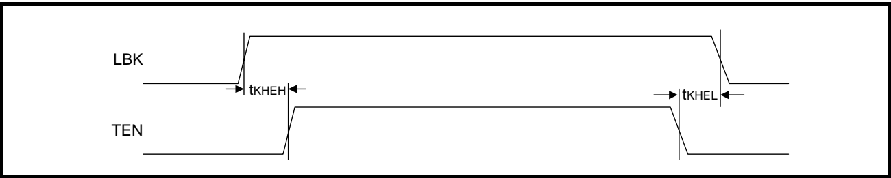
Figure 21: Mode 1 Loopback Timing
