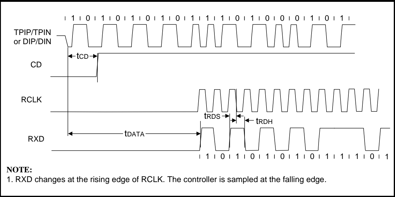
Figure 28: Mode 3 RCLK/Start-of-Frame Timing ( LXT901 only )
