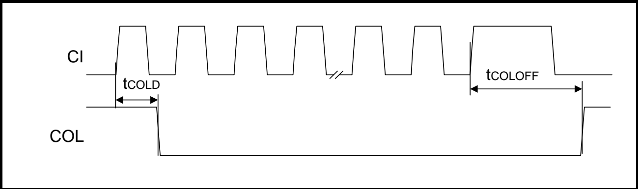
Figure 33: Mode 3 Collision Detect Timing
