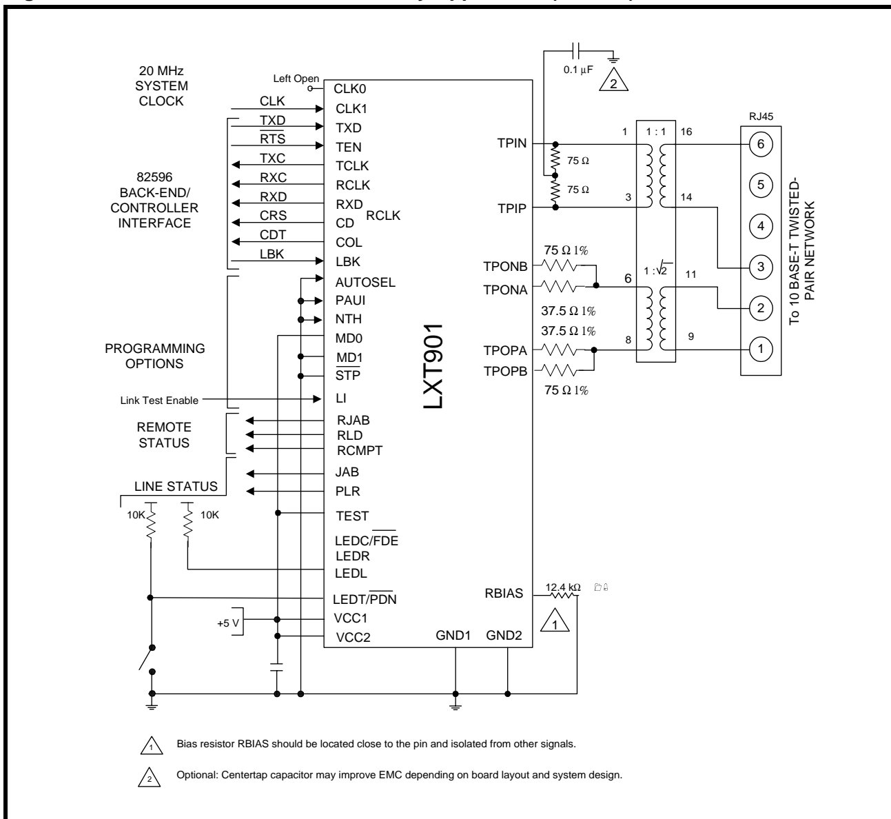
Figure 15: 150 \Omega Shielded Twisted-Pair Only Application (LXT901)
