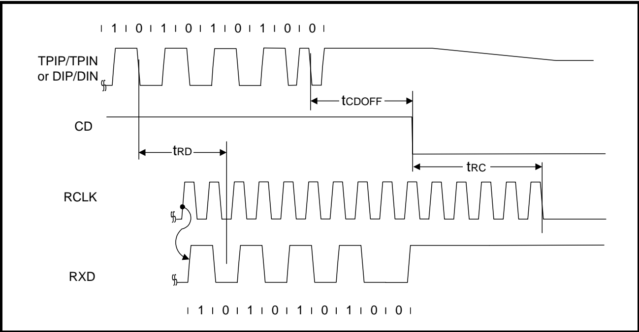
Figure 17: Mode 1 RCLK/End-of-Frame Timing
