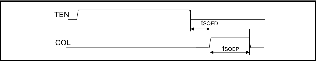
Figure 20: Mode 1 COL/CI Output Timing
