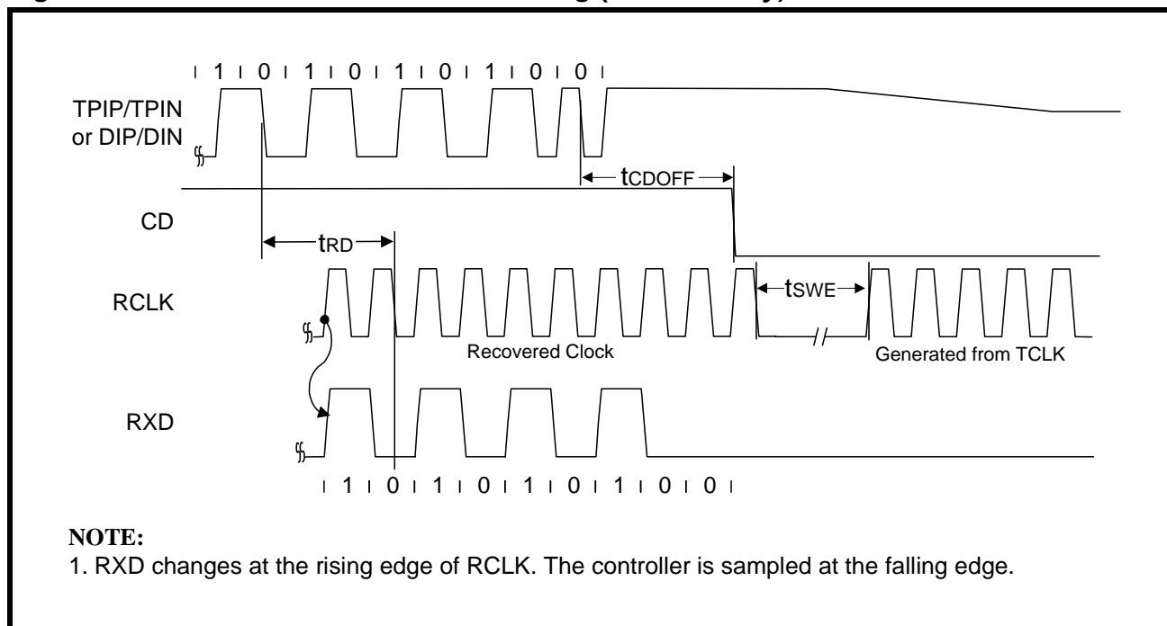
Figure 31: Mode 3 RCLK/End-of-Frame Timing (LXT907 only)
