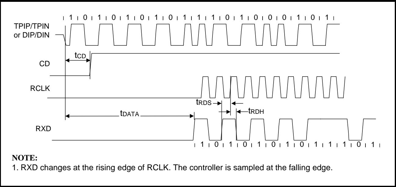
Figure 36: Mode 4 RCLK/Start-of-Frame Timing
