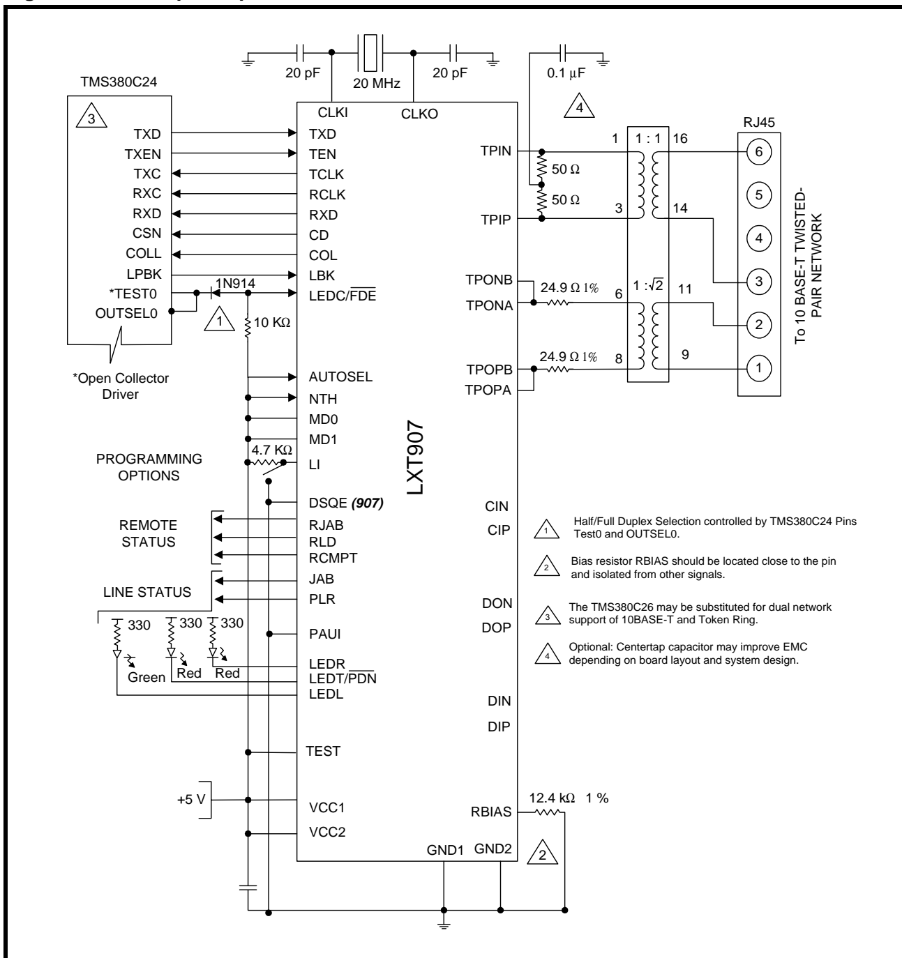
Figure 9: Full-Duplex Operation
