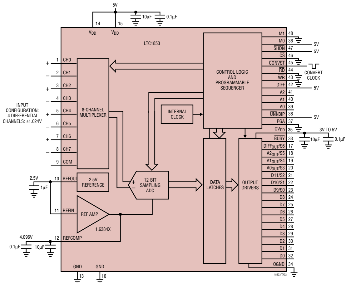
LTC1853 Hardwired for 4-Channel Differential Scan with Bipolar \pm 1.024\text{V} Operation
