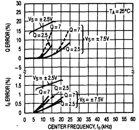
Graph 3. Mode 3, ( f_{CLK}/f_o ) = 50:1
