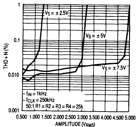
Graph 7. Total Harmonic Distortion vs Output Amplitude
