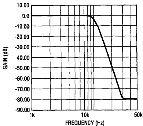
Graph 9. LTC1164 8th Order Butterworth, f_{CLK} = 500\text{kHz} , f_{-3dB} = 10\text{kHz}
