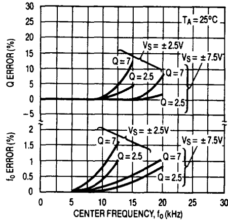
Graph 2. Mode 1, ( f_{CLK}/f_o ) = 100:1
