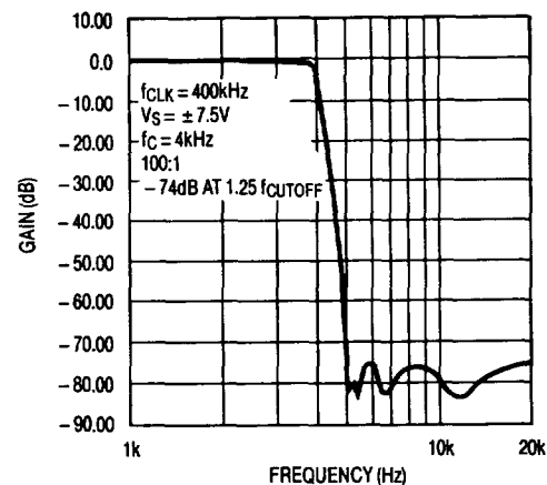
Figure 16. LTC1164 9th Order Lowpass Elliptic, f_{CUTOFF} = 4kHz
