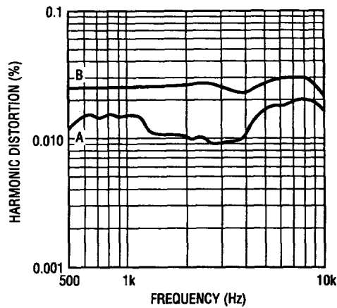
Graph 10. LTC1164 8th Order Butterworth, f CLK = 500kHz, f -3dB = 10kHz ±8V, A. 2V RMS , B. 4V RMS
