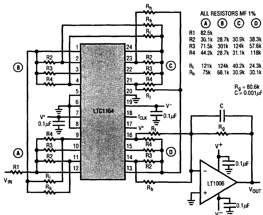
Figure 15. LTC1164 9th Order Lowpass Elliptic, Fixed f_{CUTOFF} = 4kHz , f_{CLK} = 400kHz , -74dB at 5kHz , Passband Noise = 210\mu V_{RMS} \pm 5V
