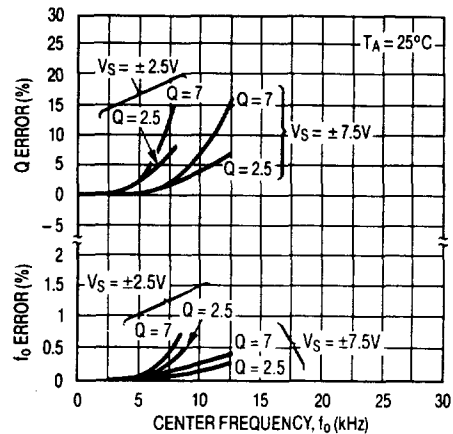
Graph 4. Mode 3, ( f_{CLK}/f_o ) = 100:1
