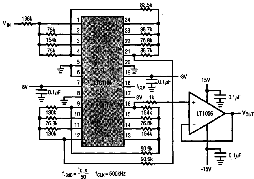
Figure 11. 8th Order Lowpass Butterworth, Passband Noise 90\mu\text{V}_{\text{RMS}} (Also Refer to the LTC1164-5)
