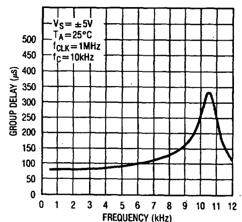
Graph 3. Group Delay
