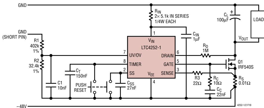
Figure 19. -48V/5A Application
