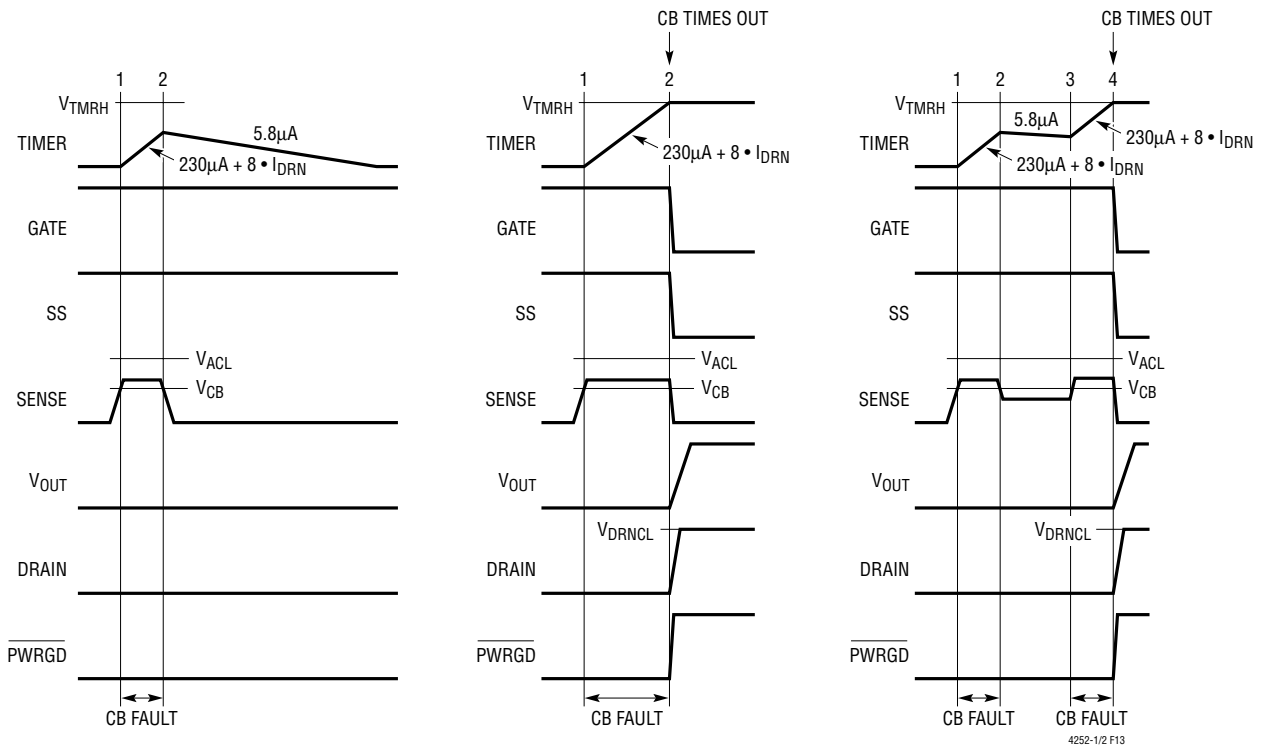
Figure 13. Circuit-Breaker Timing Behavior (All Waveforms are Referenced to V_{EE} )
