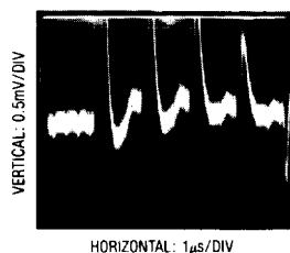
Figure 16. Poor Reference Settling Can Cause A/D Errors
