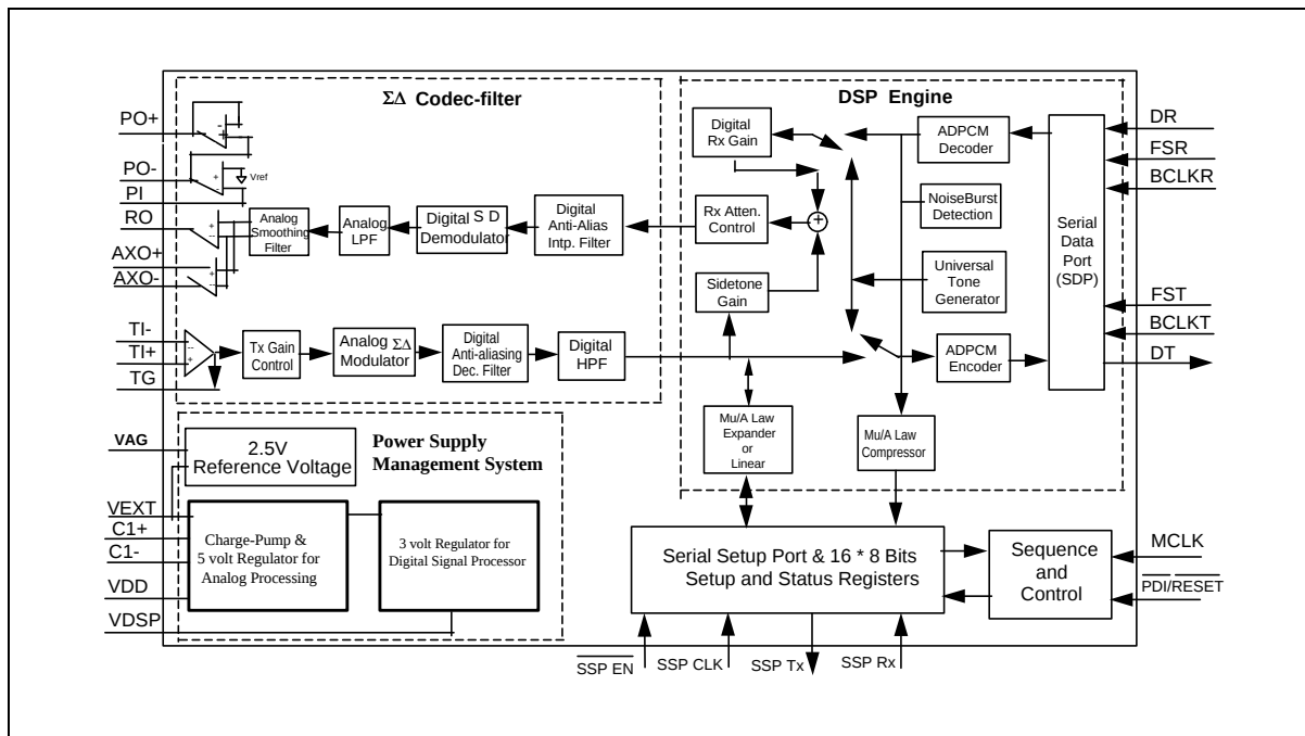
Figure 6-1 Lanwave ADPCM \Sigma\Delta Codec Block Diagram
