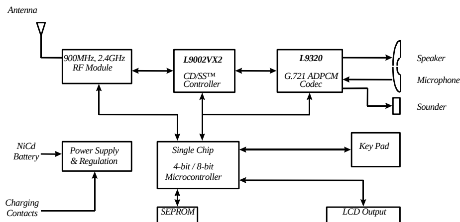
Figure 5-2 System Diagram for Cordless Phone Application
