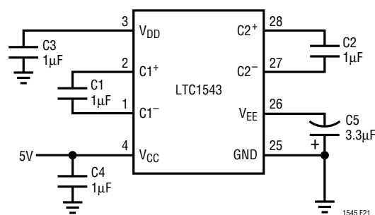
Figure 21. Charge Pump
